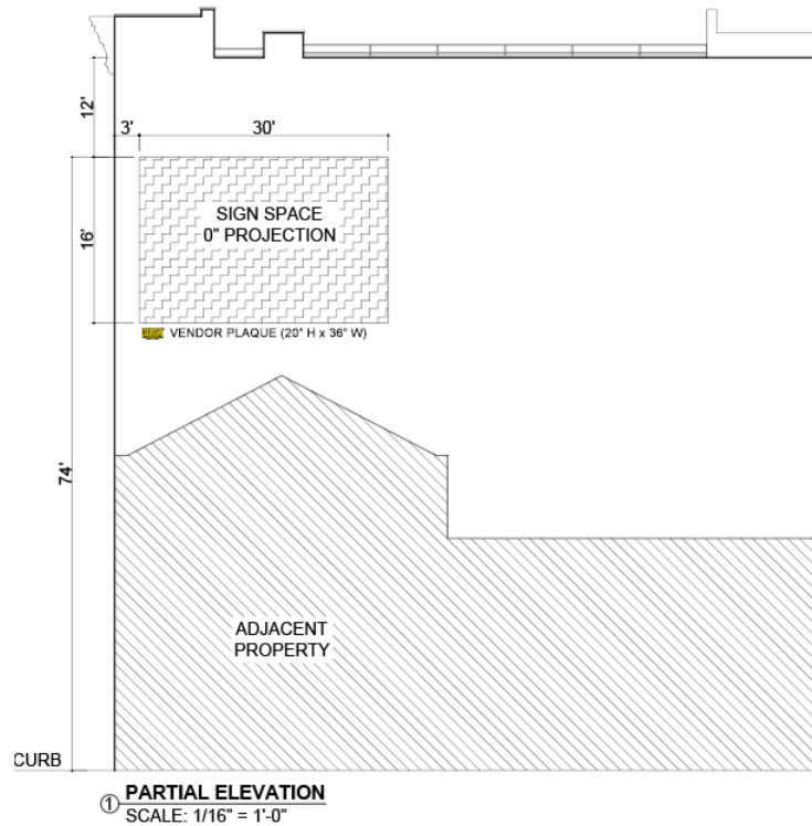
Architectural Elevation
